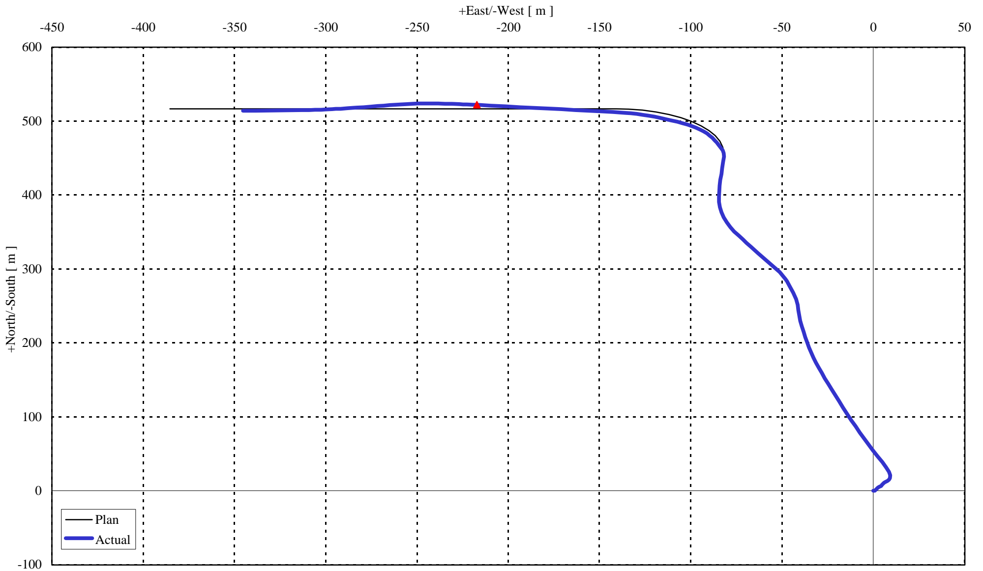
Example Well - Comparison "Plan" vs. "Actual" Horizontal Projection
